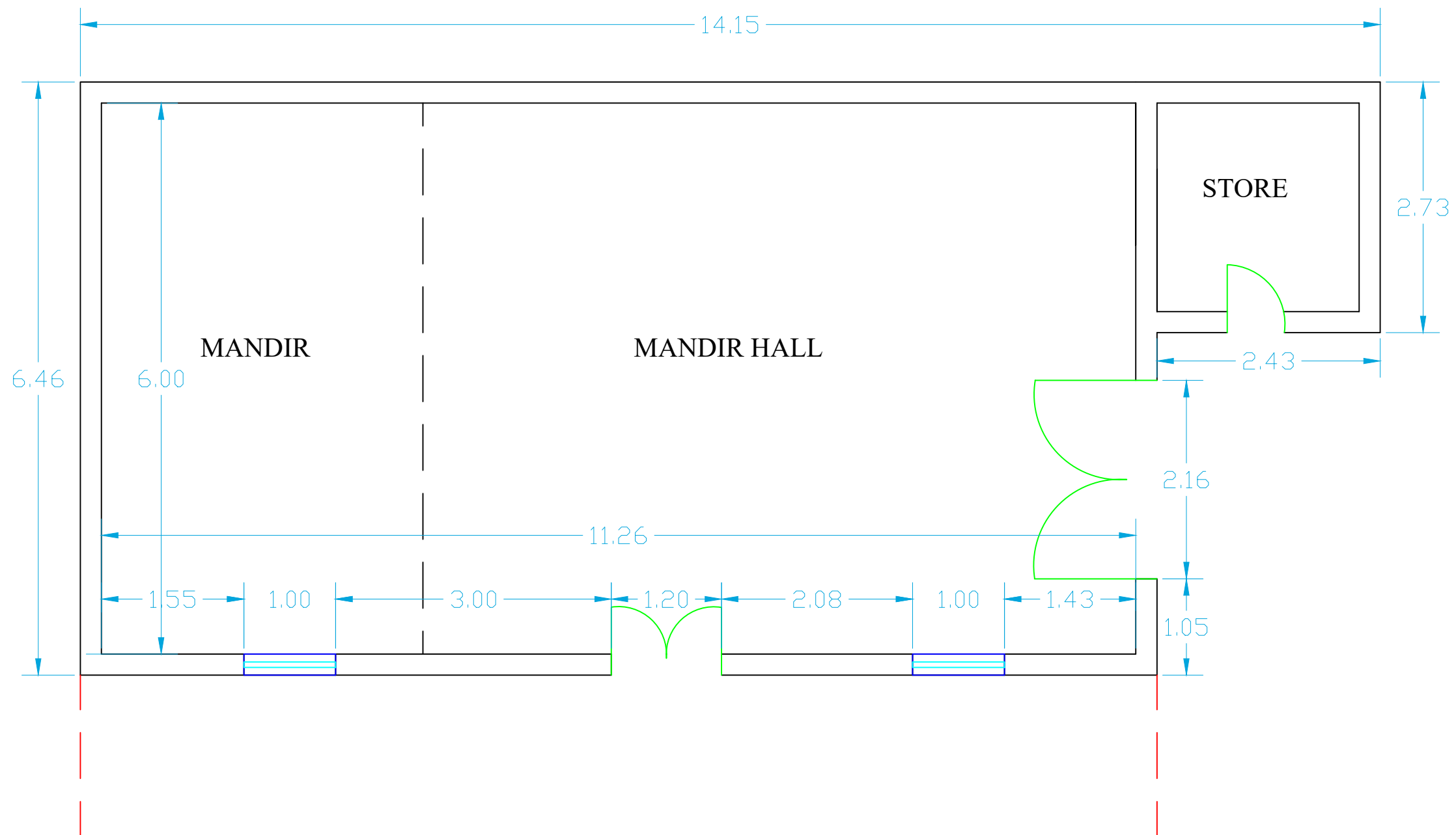
MANDIR BLOCK - GROUND FLOOR
